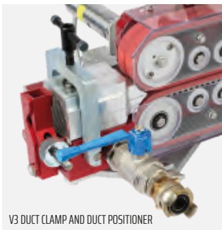
V3 DUCT CLAMP AND DUCT POSITIONER
